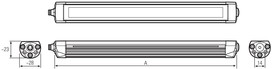
TUBELED_25: 154x10-01
