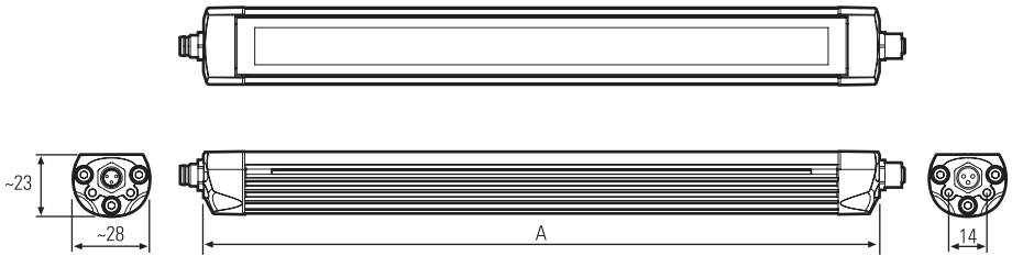
TUBELED_25: 154x10-02
