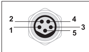
Schematic drawing of M8 plug
