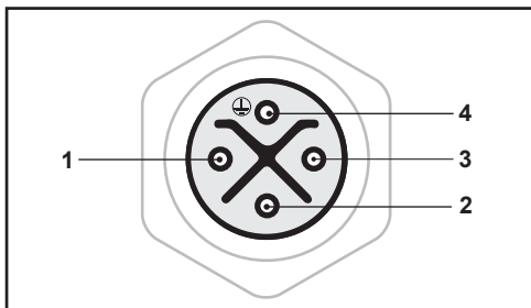
Schematic drawing of M12 plug, S-coded
