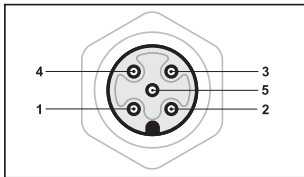
Schematic drawing of M12 plug
