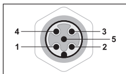
Schematic drawing of M12 plug
