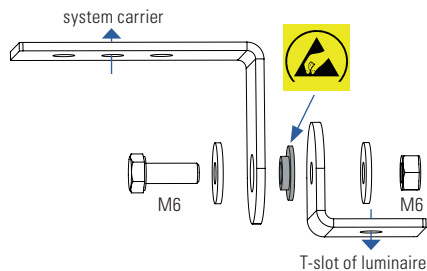
mounting kit, optional: 240400-02
