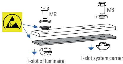
mounting kit, optional: 240400-01
