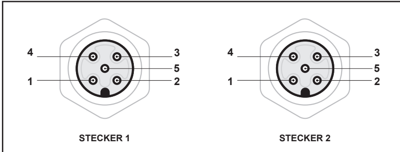
Schematic drawing of M12 connectors
